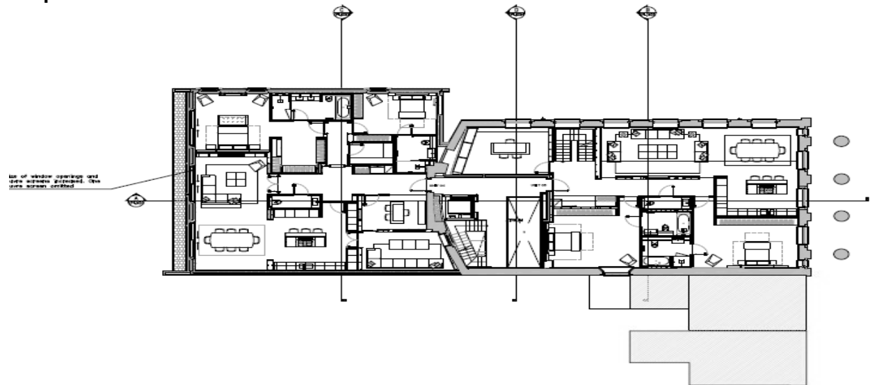
Proposed Second Floor Plan
